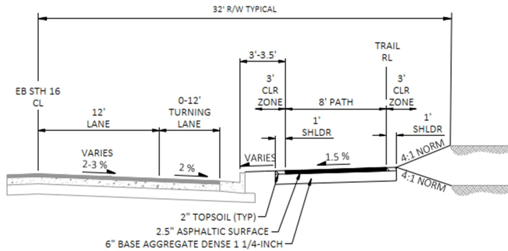
FINISHED TYPICAL SECTION
